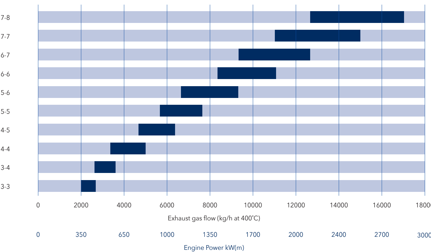
For indication only, please contact us for exact unit selection or custom solutions. Bars in graph correspond with 20-30 mbar pressure drop.
