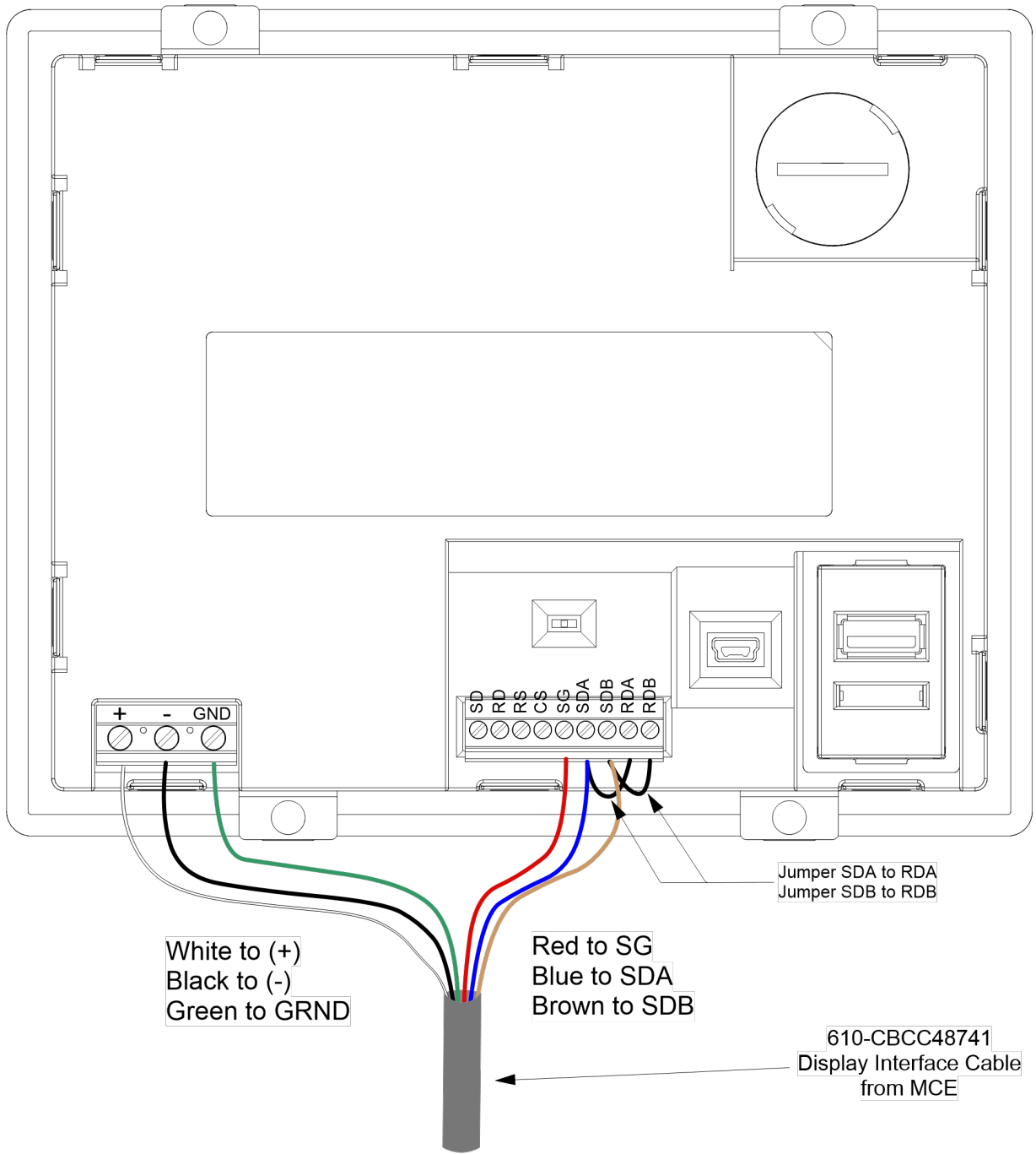
Power and Data wiring for the 610-FCI-T4N Touch Screen / Display RS 485 Connection to MCE (Older)
