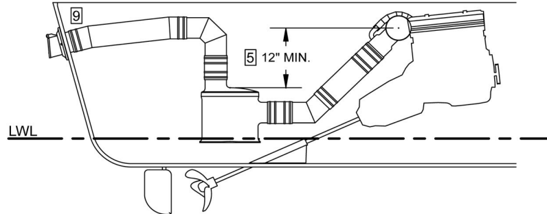
FIG. 1 ENGINE INSTALLATION ABOVE WATERLINE
